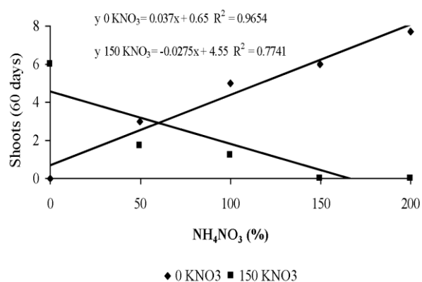
Fig 2. Effect of nitrogen concentrations in MS medium on the formation of shoots in explants of cotyledon leaves of physic nuts ( Jatropha curcas ) cultured in vitro for 60 days after inoculation. (A) Interaction between concentrations of \text{NH}_4\text{NO}_3 with \text{KNO}_3 on the number of shoots. (B) Interaction between concentrations of \text{KNO}_3 with \text{NH}_4\text{NO}_3 on the number of shoots.
