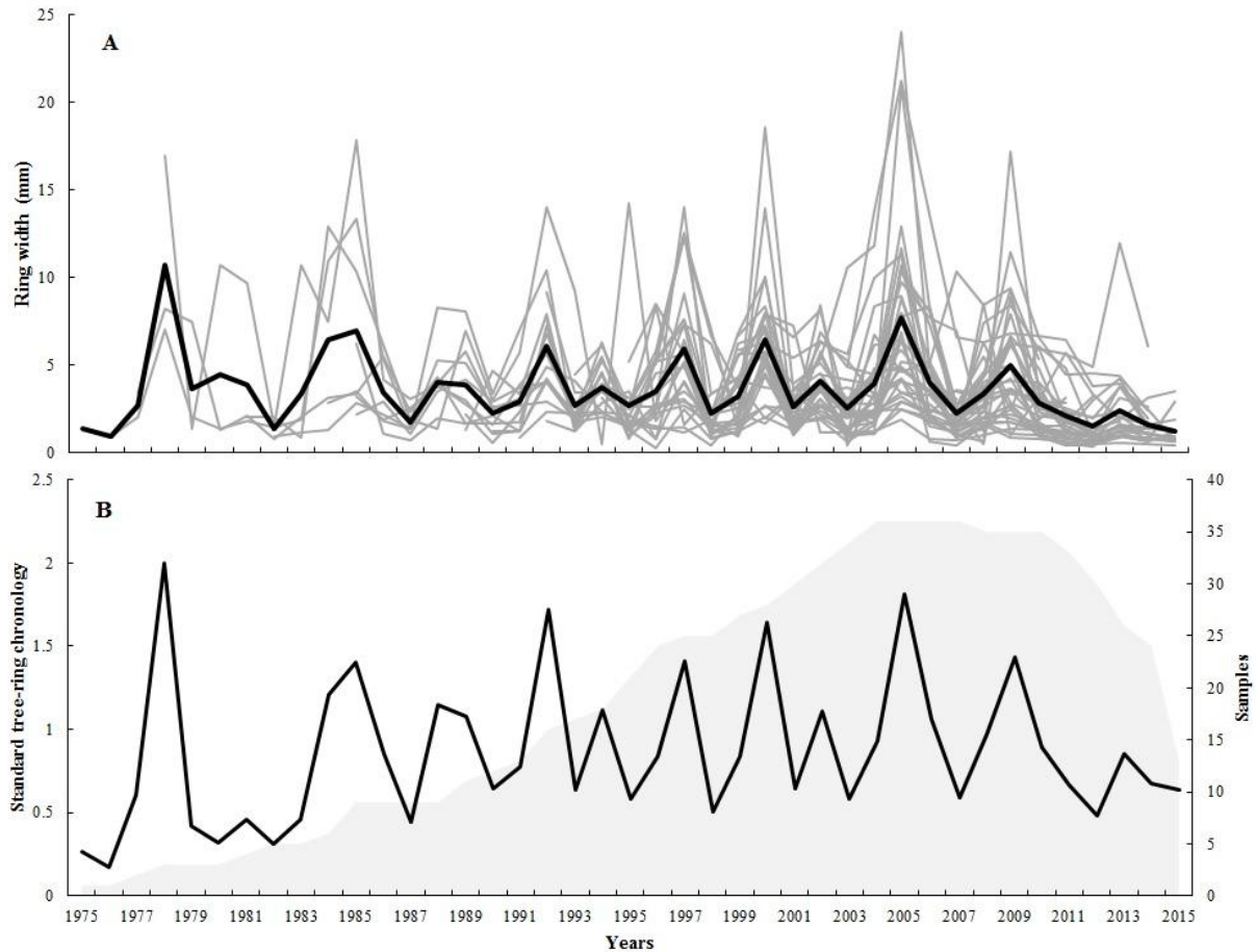
Fig. 2.2.5: (A) Radial measurements of the growth rings of Prosopis juliflora (gray lines) and the mean values (black line). (B) Standard chronology of P. juliflora and the number of samples that contributed to the chronology in each year (area).
