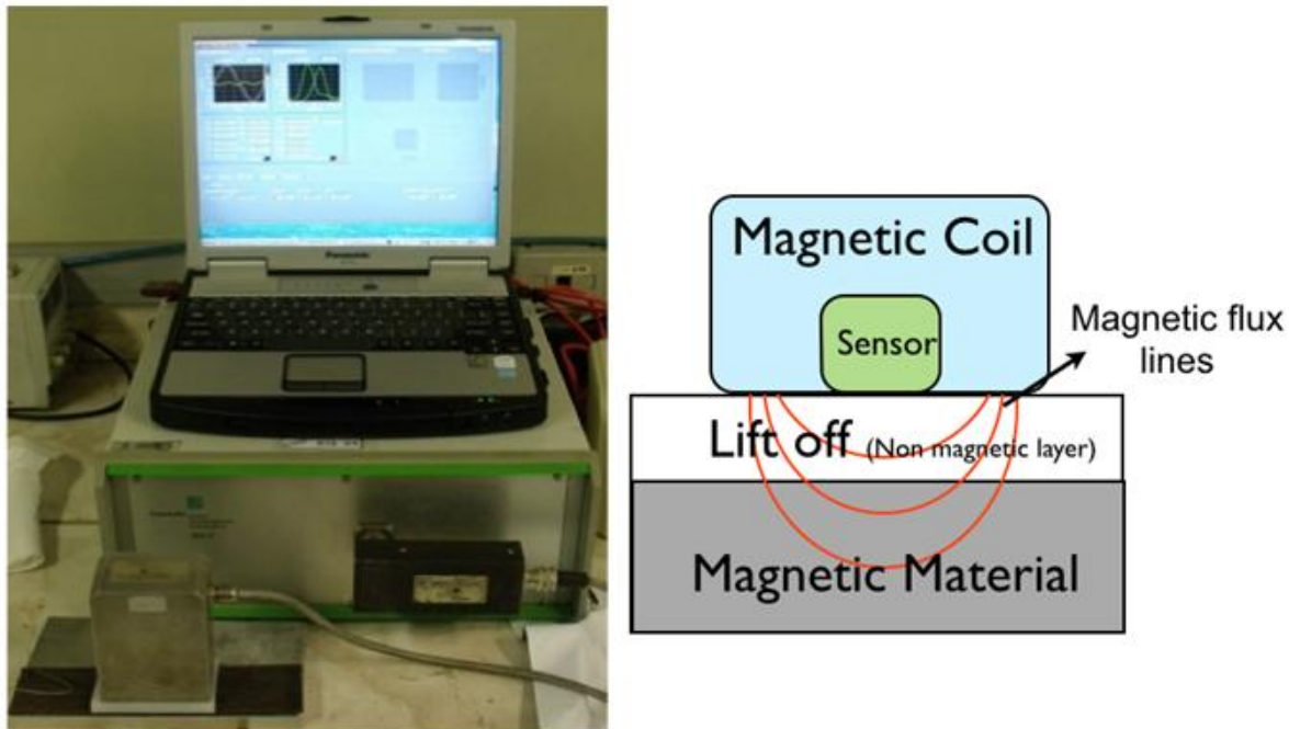
Figure 2. 3MA-II equipment and schematic of the experimental setup adopted for the measurements.
